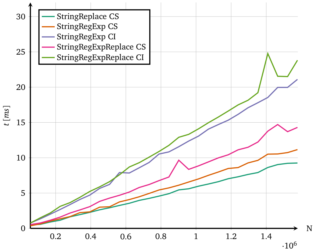
Performance of substring count AI v.3.3.8.1 x86
