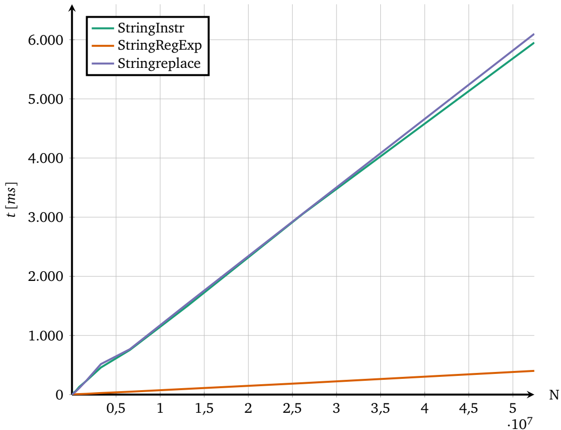
Performance of substring count AI v.3.3.8.1 x86
