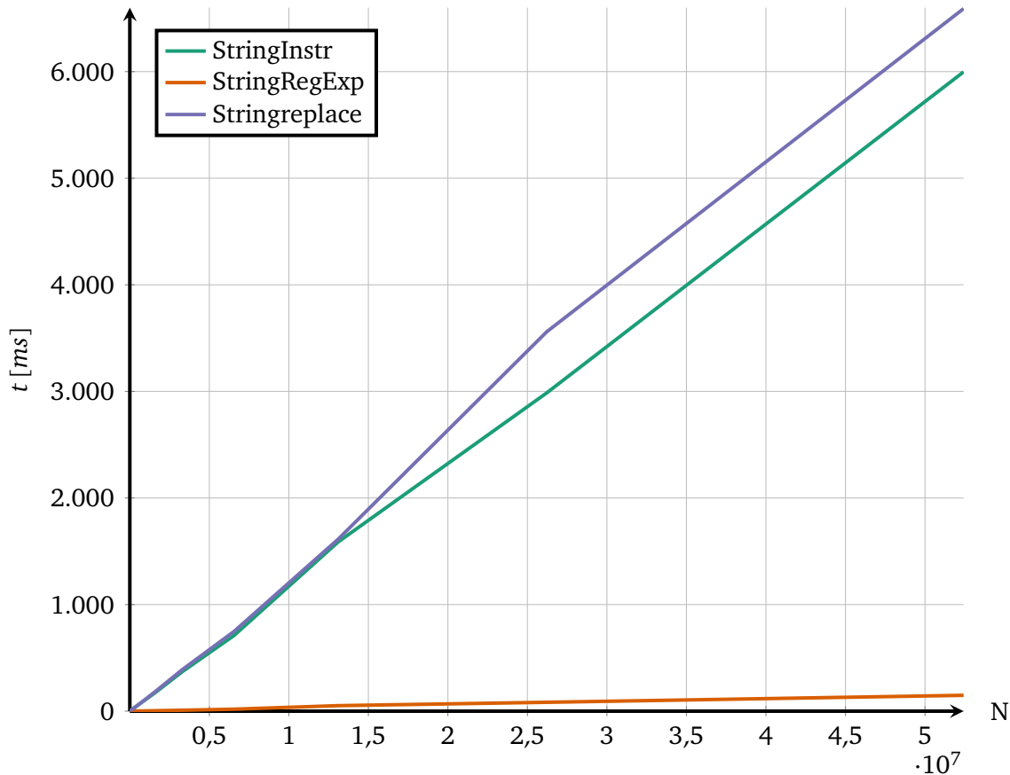
Performance of substring count AI v.3.3.12.0 x86
