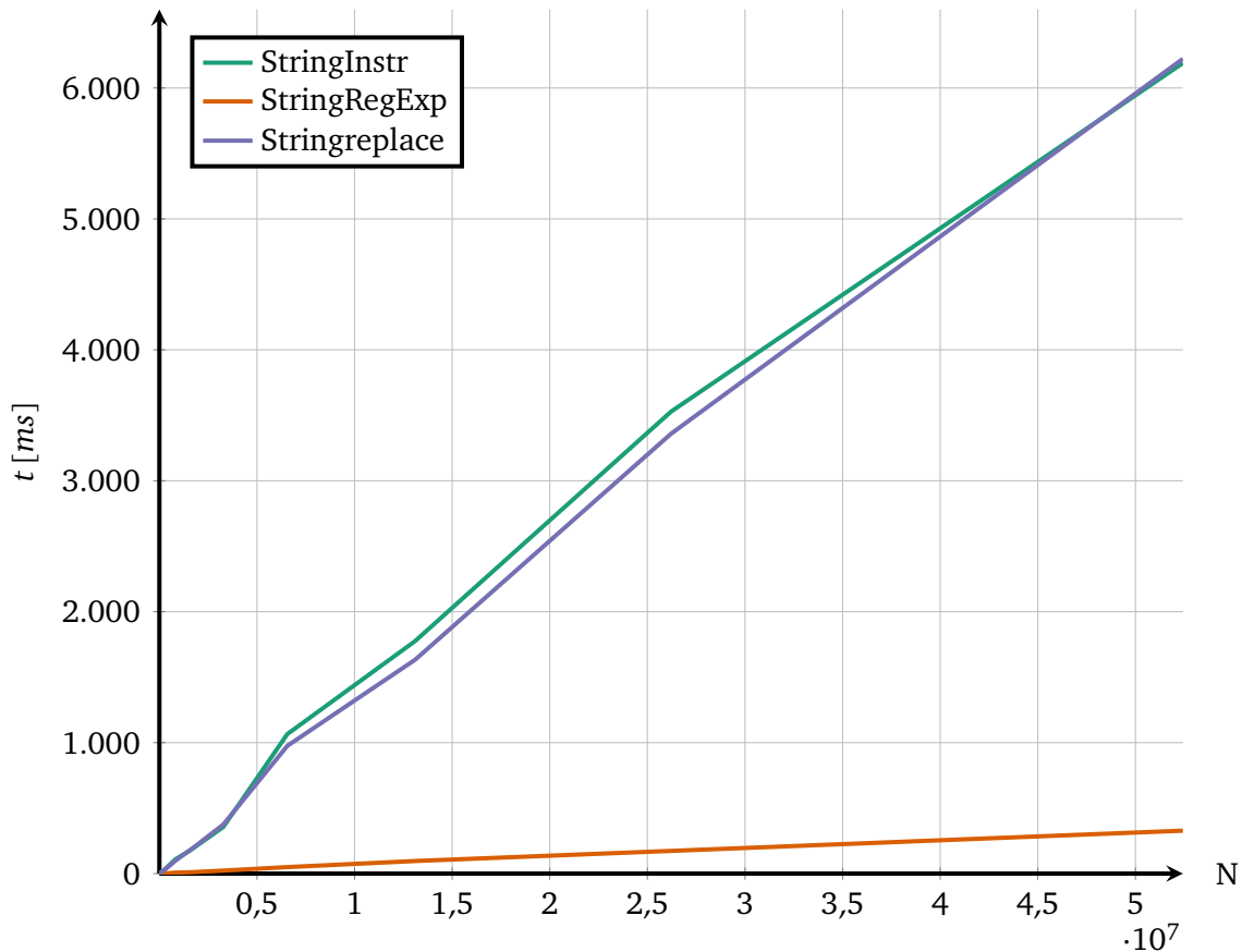
Performance of substring count AI v.3.3.6.0 x86
